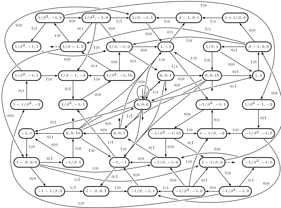
Figure 9. Normalizing transducer \mathcal{N}_\beta , \beta^3 = \beta^2 + \beta + 1 .
