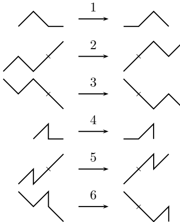
FIGURE 13. Effect of transforming some NES peaks into NESE peaks in the path from Figure 12. In this example, \lambda = (5, 4, 3, 1) .
