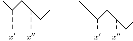
FIGURE 18. The relative height of p remains one when we apply the operation 3 or 6.
