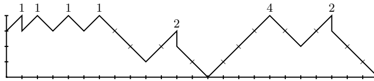
FIGURE 13. Effect of transforming some NES peaks into NESE peaks in the path from Figure 12. In this example, \lambda = (5, 4, 3, 1) .
