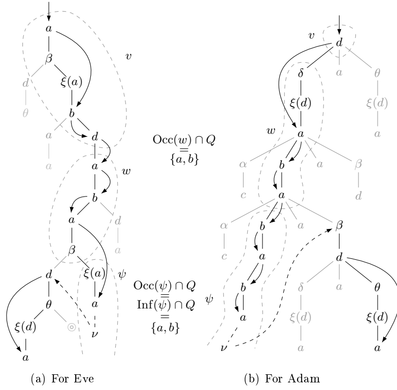
Fig. 4. Strategy translation from \mathbb{G} to G
