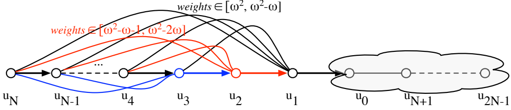
Figure 1: The graph G_n in the proof of Theorem 1.
