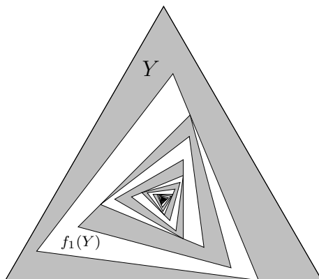
FIGURE 5. A dissection of the triangle with area ratio 1 : 2. The dissection is done by the IFS \{f_1\} with f_1(x, y) = \sqrt{1/2}R(5\pi/8)(x, y) + (4/5, 0) where R(\alpha) denotes the counterclockwise rotation with angle \alpha ; Y = \overline{D \setminus f_1(D)} .
