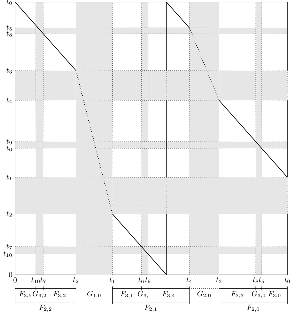
FIGURE 3. The (-\beta) -transformation for \beta = 9/8 with gaps G_{m,k} , support of the invariant measure F_{3,0} \cup \dots \cup F_{3,5} , and t_k = T_{-\beta}^k(1) . Ratios between G_{1,0} , G_{2,0} and the rest of the picture are not respected. In reality, G_{1,0} is almost 10 times the size of G_{2,0} , and G_{2,0} is almost 5 times the size of F_{2,0} .
