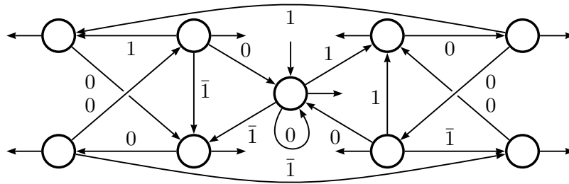
FIGURE 1. Automaton recognising the set of F -expansions of minimal weight in \{-1, 0, 1\}^* .
