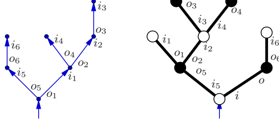
Figure 10: A pair (A, B) coherently labelled on the alphabet \{i, i_1, \dots, i_6, o, o_1, \dots, o_6\} : the face-permutation \varphi of the tree A satisfies \varphi|_{O'} = (o, o_1, \dots, o_6) , while the face-permutation \psi of the mobile B satisfies \psi|_{I'} = (i, i_1, \dots, i_6) .
