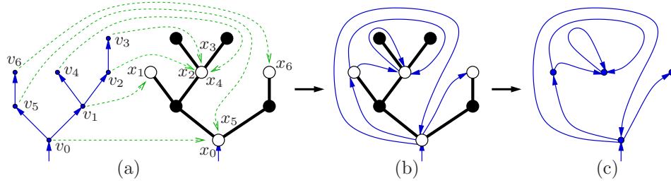
Figure 11: Topological representation of the folding step. Figure (b) represents the partially folded map.
