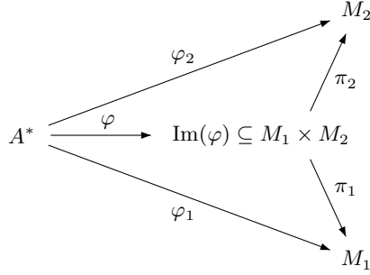
Figure 2.1: The restricted direct product of two stamps.
