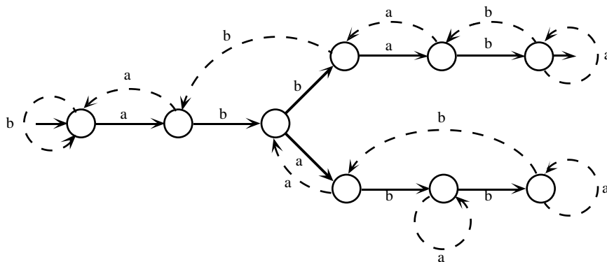
Figure 3.2. A possible completion.
