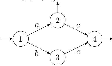
Figure 2.5: The minimal automaton of \{a, ac, bc\} .
